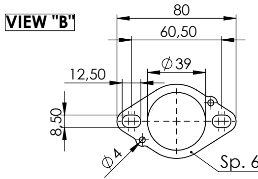
Flange "158A" Cod.206061
