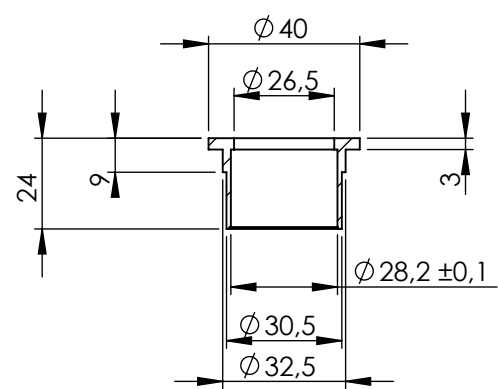
S.s. bushing cod.206662
